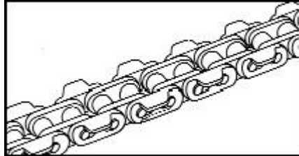
SFB/L - Side Flexing Black, 'L' shaped sideplate
